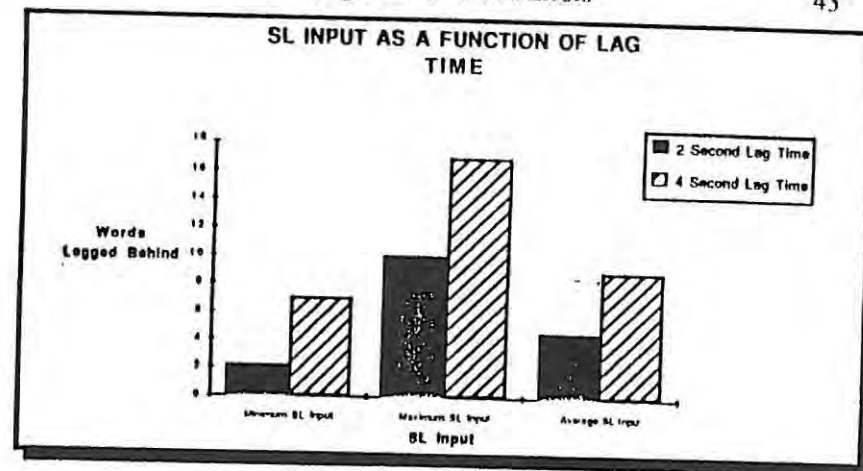
Figure 1. Source language input as a function of lag time.
