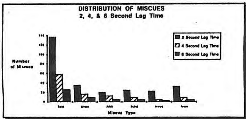
Figure 11. Distribution of miscues by 2, 4, and 6-sec. lag time.
